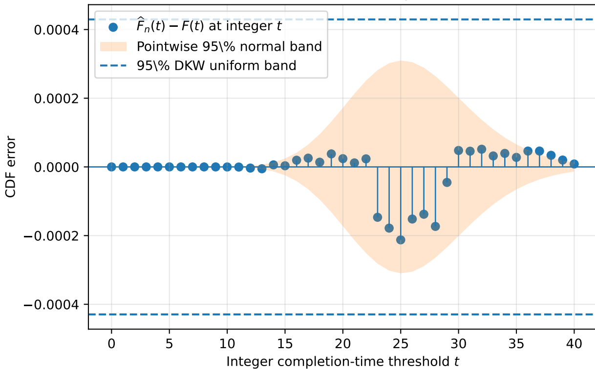
Monte Carlo CDF error at integer thresholds
